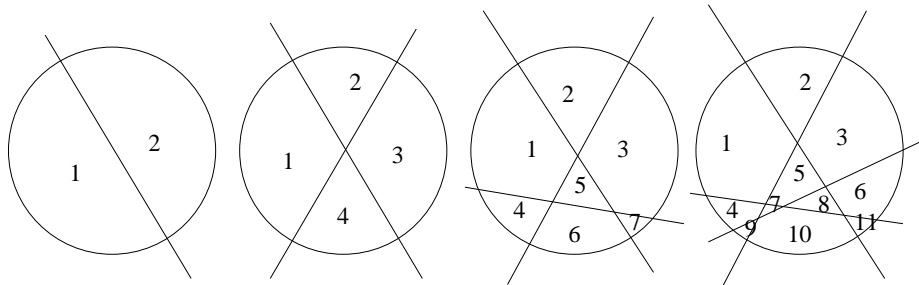
FIGURE 1. Plane regions.
